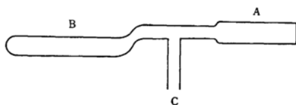
Fig. 1. Reaction cell. Part A. Thickness 10 mm. plane parallel. Part B. Diameter ca. 12 mm. (painted with black enamel).
