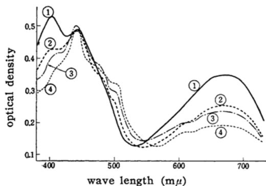
Fig. 3. Change of absorption spectra (visible light irradiation). Methylene blue ca. 4 \times 10^{-5}\text{M} \text{H}_2\text{SO}_4 22.9 N Alcohol 4.96 M ① — initial ② --- after 1 hr. irradiation ③ - - - after 2.5 hr.' irradiation ④ ..... after 5.5 hr.' irradiation
