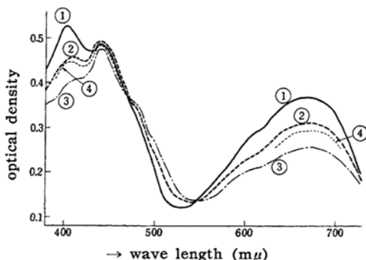
Fig. 2. Change of absorption spectra (visible light irradiation). Methylene blue ca. 4 \times 10^{-5}\text{M} \text{H}_2\text{SO}_4 22.9 N Alcohol 3.38 M ① — initial ② --- after 3.5 hr.' irradiation ③ - - - after 8 hr.' irradiation ④ ..... exposed to oxygen after irradiation
